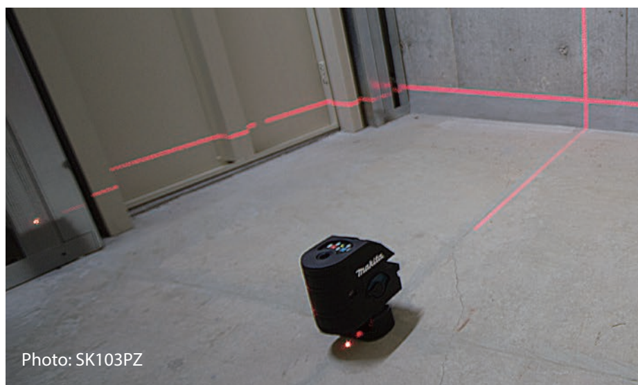
Photo: SK103PZ with Adapter (magnetic)
